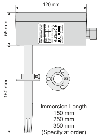
EHTC-DC-xV-x50-xx-xx DUCT TYPE
